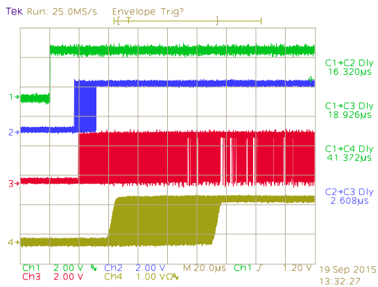
Fig. 11: Accumulated samples of motion-to-photon latency measurement. Same channel labels as Figure 10. Delay times at the right are the minimums of those captured. In this aggregate example, total latency (C1→C4) ranged between 41.372 \mu s and about 115 \mu s.
