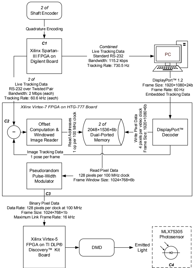
Fig. 3: Implemented data path framework. Labels C1-C4 indicate oscilloscope channels assigned to measurement test points used during latency analysis. The photosensor ( C4 ) is present and used only during latency testing.
