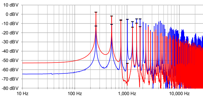
Fig. 9: Spectra of 6-bit PWM (red) and PR-PDM (blue) simulated signals from Figure 8(a). For clarity, the local maximums of the first several harmonics are highlighted with dash marks of the same color.
