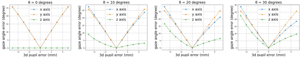
Figure 3: The correlation between 3D pupil center error and gaze angle error at 0°, 10°, 20°, and 30° horizontal gaze angle.
